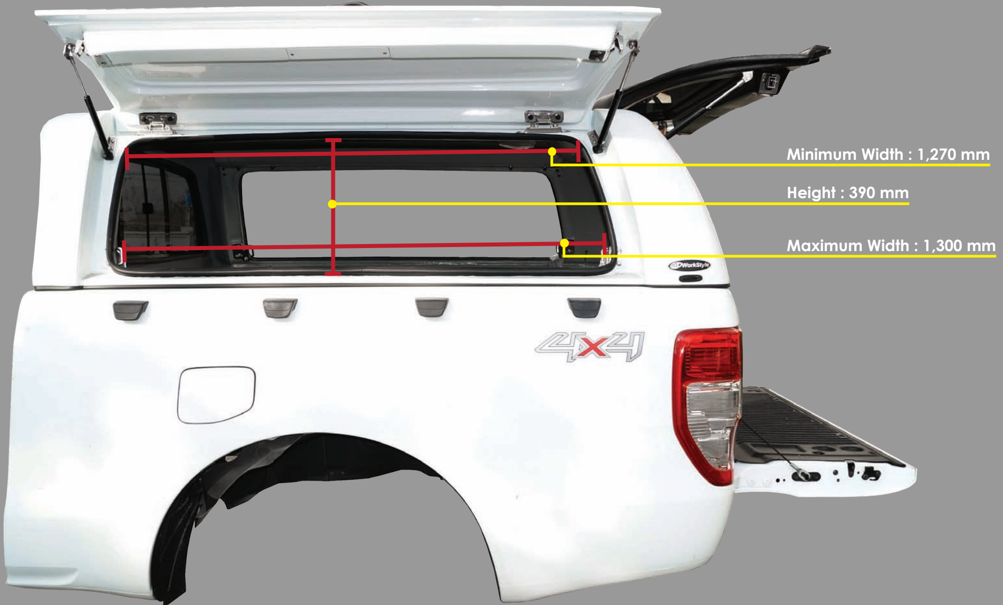
New 2012+ Ford Ranger.MK.5 (PX Ranger/T6) Extra-Cab
